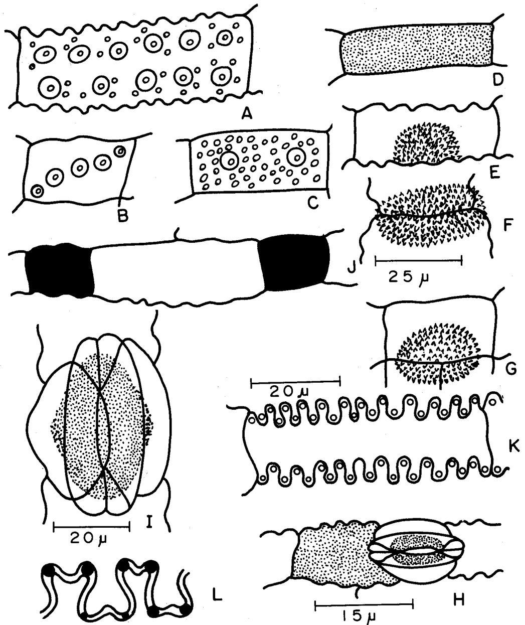
Fig. 2. Distribution of silica bodies in sedges
