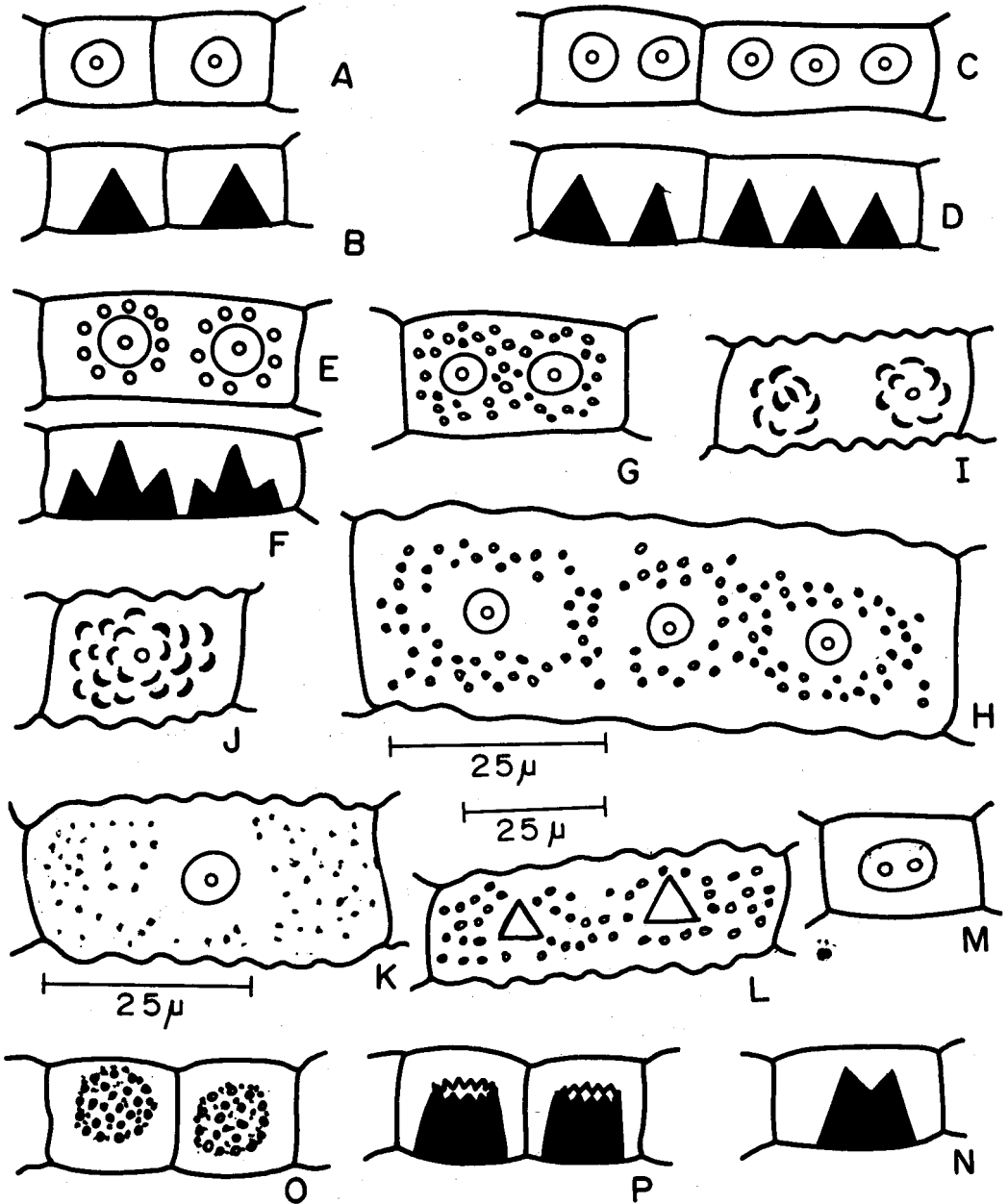
Fig. 1. Distribution of silica bodies in sedges
